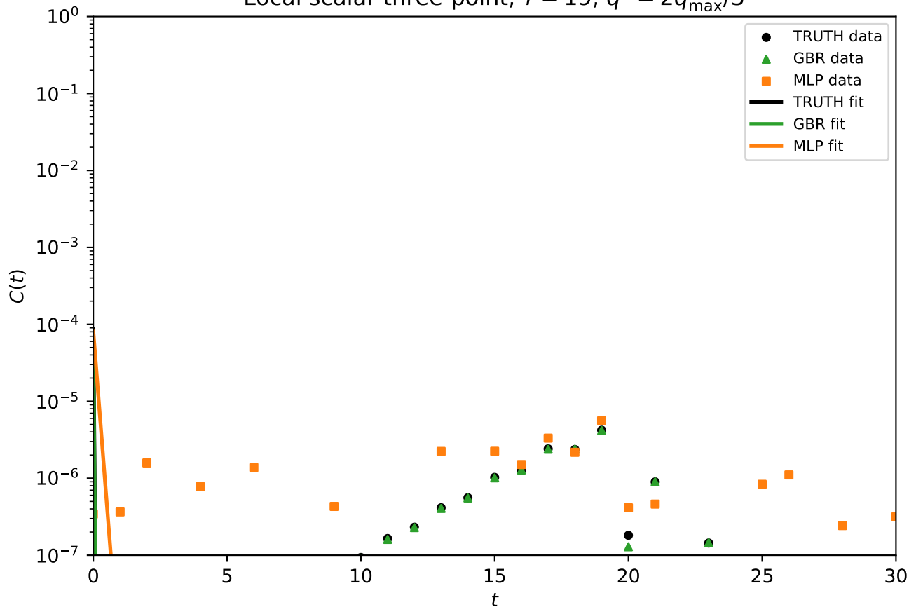
Local scalar three-point, T = 19 , q^2 = 2q_{\max}^2/3
